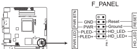
M4A88T-I DELUXE System panel connector
