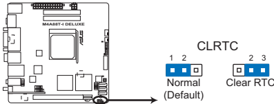
M4A88T-I DELUXE Clear RTC RAM
