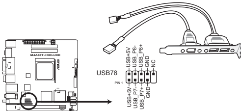
M4A88T-I DELUXE USB2.0 connector
