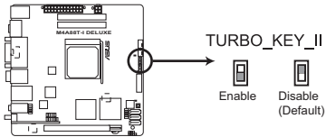
M4A88T-I DELUXE Turbo Key II Switch
